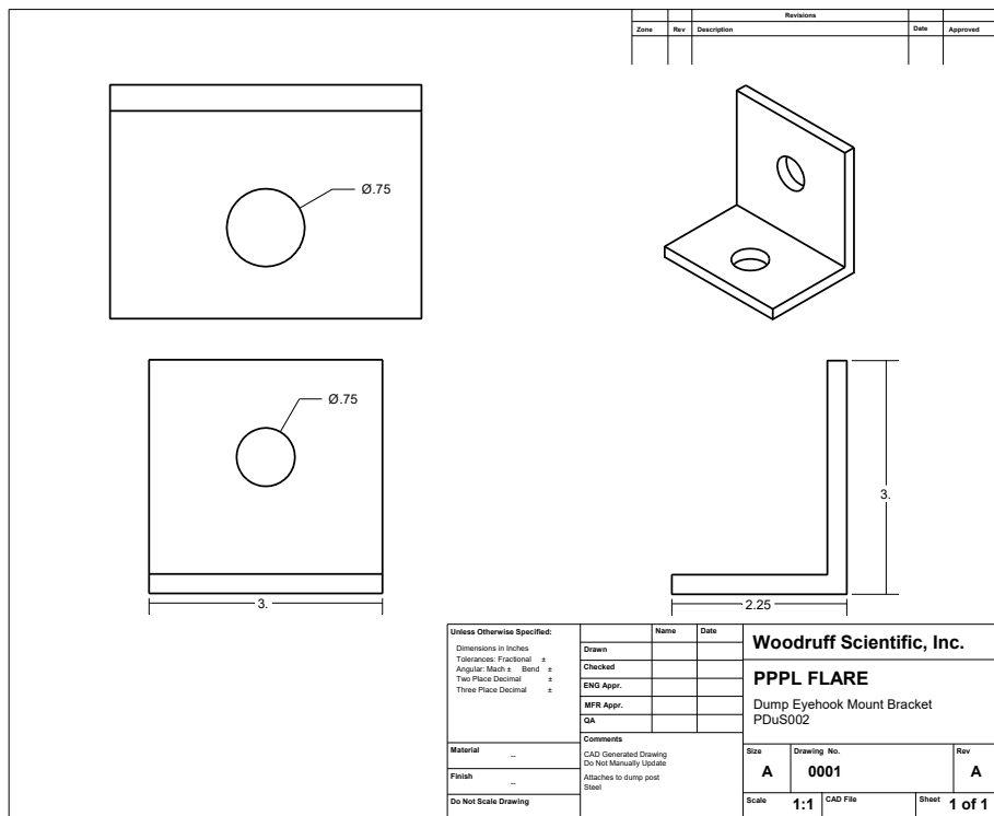
Figure 23: Dump Stick Eyehook Bracket
