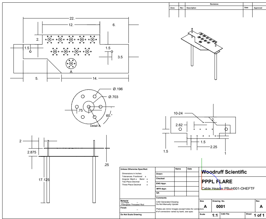
Figure 21: PF Cable Header
