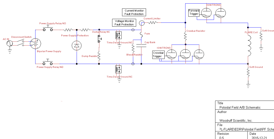
Figure 1: Poloidal Field Circuit Schematic
