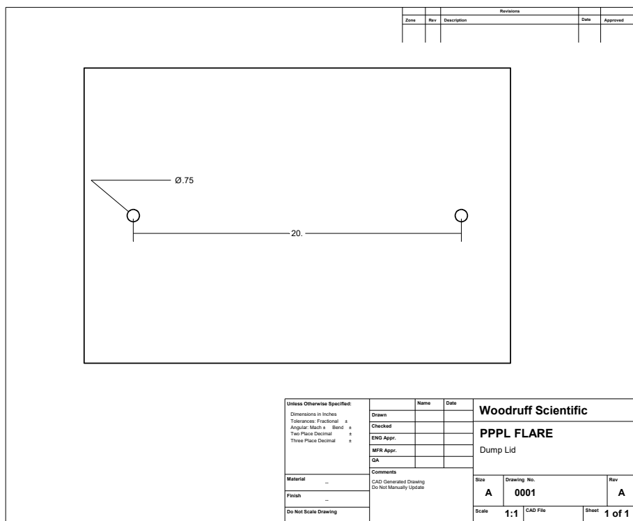
Figure 22: Dump Lid
