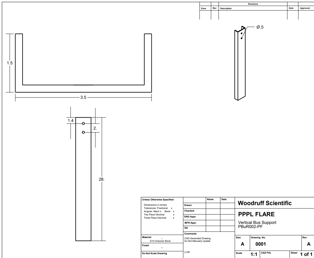
Figure 17: PF Bus Vertical Support - 2 Off
