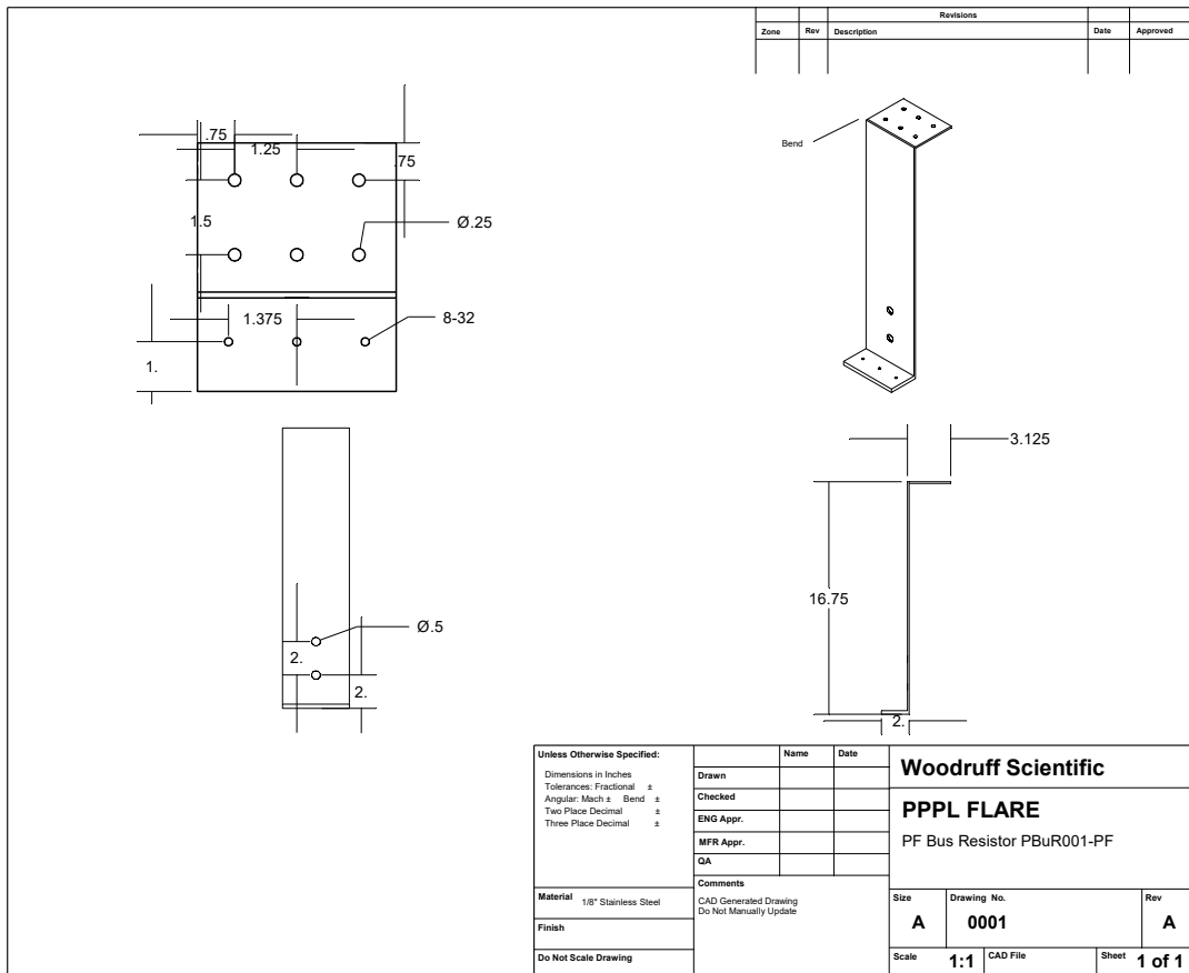
Figure 19: PF Bus Resistor
