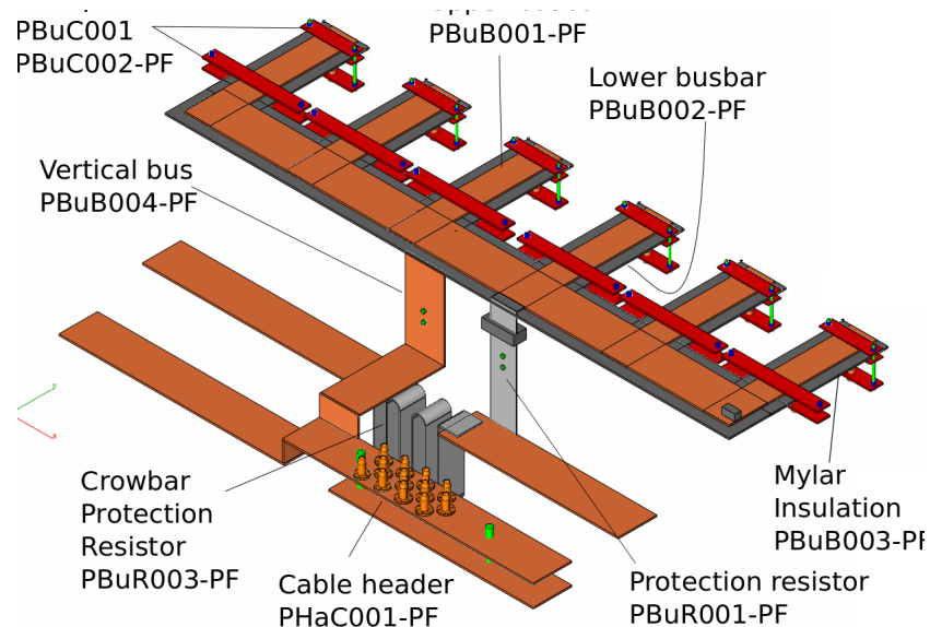
Figure 6: Buswork detail.
