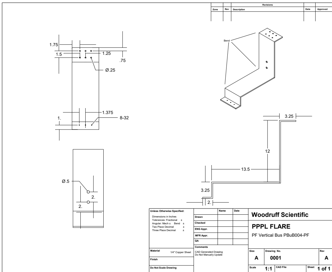
Figure 18: PF Bus Vertical
